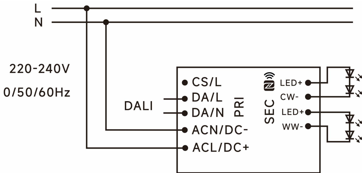
DALI Connection
